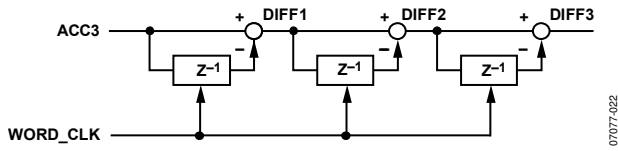
Figure 26. Differentiator
