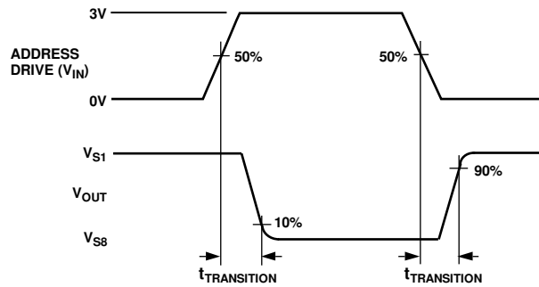
Figure 28. Switching Time of Multiplexer, t TRANSITION
