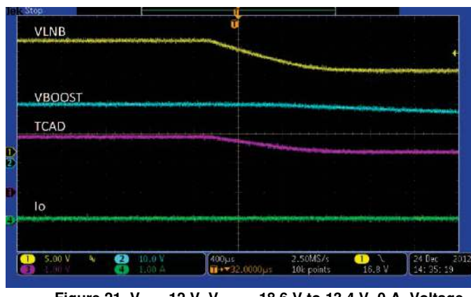
Figure 21. V_{IN} = 12\text{ V} , V_{LNB} = 18.6\text{ V to }13.4\text{ V} , 0 A, Voltage Transition
