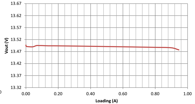
Figure 2. Load Regulation ( V_{IN} = 12\text{ V} , V_{LNB} = 13.4\text{ V} )
