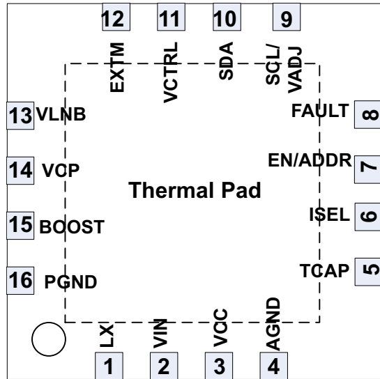
RTE PACKAGE (TOP VIEW)
