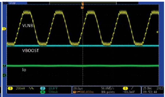
Figure 30. V_{IN} = 12\text{ V} , V_{LNB} = 18.6\text{ V} , 1\text{ A} , 22-kHz Tone
