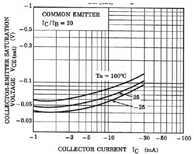
Fig. 10.22 RN2304 V_{CE(sat)}-I_C
