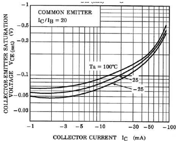
Fig. 10.23 RN2305 V_{CE(sat)}-I_C
