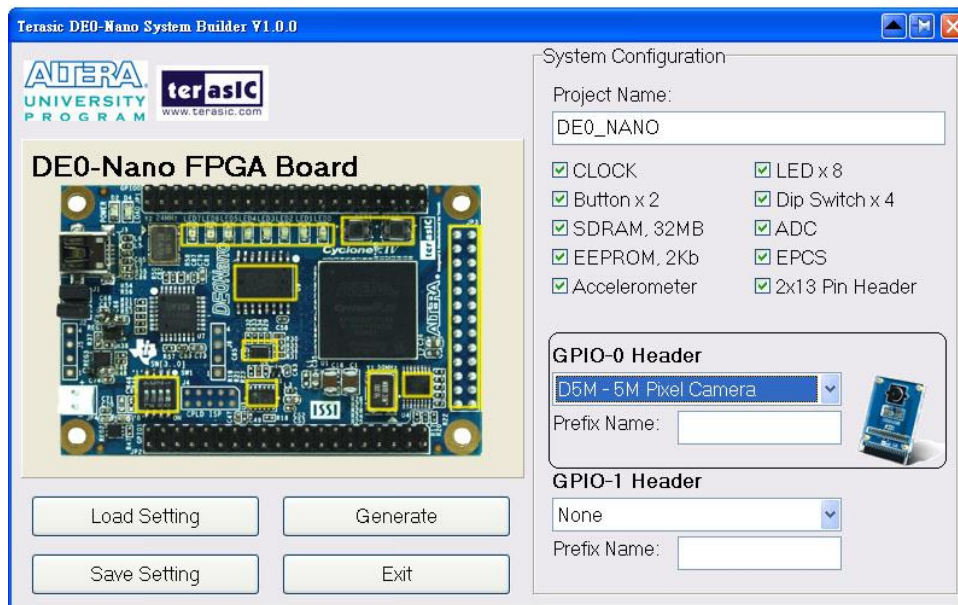
Figure 5-5 GPIO Expansion Group
