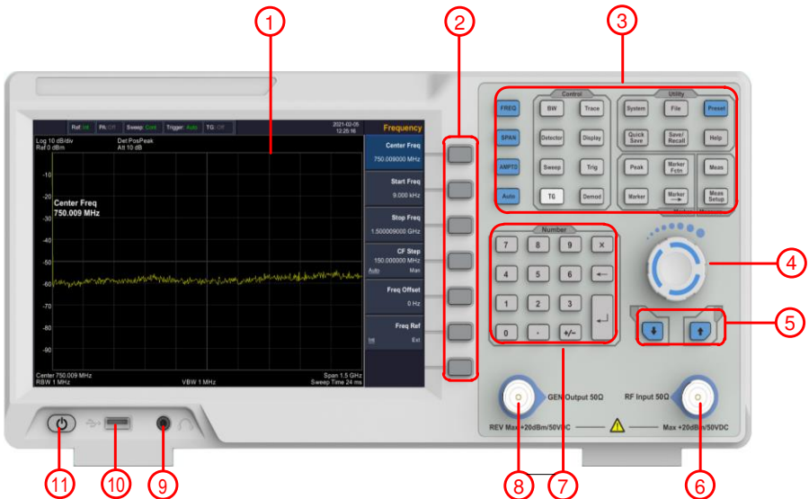
Figure 3-1 Front panel
