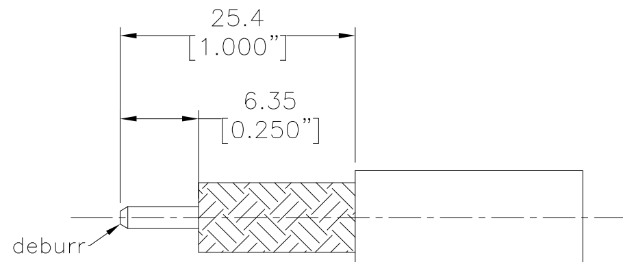
RECOMMENDED CABLE STRIPPING DIM'S Connector Adds: 36.95 mm
