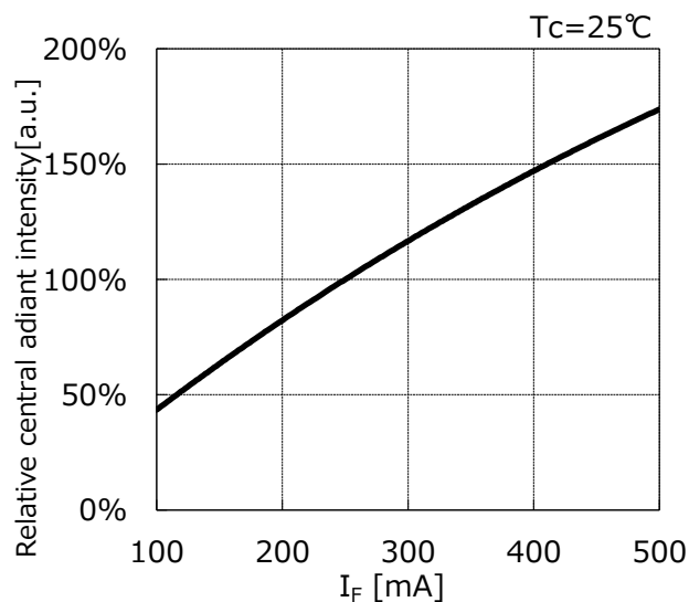
◆ Forward Current – Relative Central radiant intensity Characteristics
