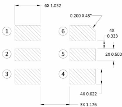
Example Land Pattern
