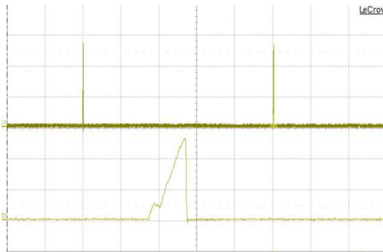
Fig. 17: Load current (top trace, 10 A/div., 100 ms/div.) into a 10 m \Omega short circuit during restart, at V_{in} = 48 V. Bottom trace (10 A/div., 10 ms/div.) is an expansion of the on-time portion of the top trace.
