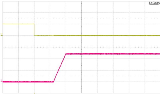
Fig. 9: Turn-on transient at full rated load current (resistive) with C_{out} 10 \mu F tantalum + 1 \mu F ceramic at V_{in} = 48 V, triggered via ON/OFF pin. Top trace: ON/OFF signal (5 V/div.). Bottom trace: output voltage (5 V/div.). Time scale: 50 ms/div.
