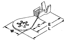
F Anti-Rotational
