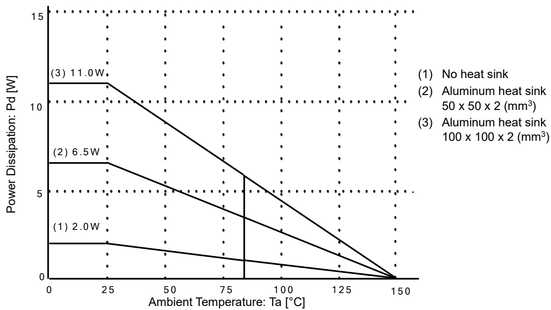
Figure 17. Power Dissipation
