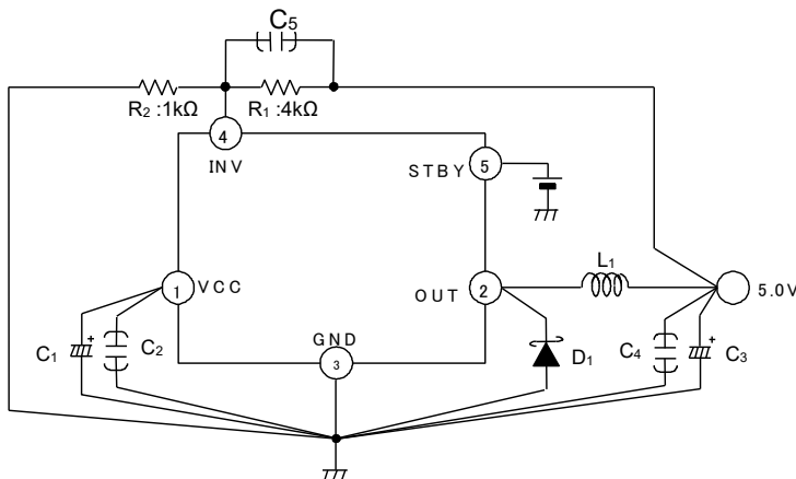
Figure 13. Layout
