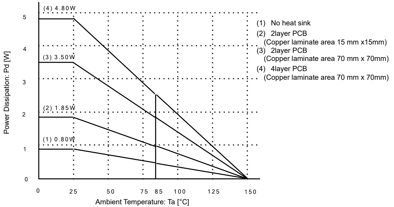
Figure 16. Power Dissipation
