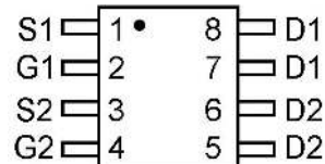
pin assignment
