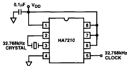
32.768kHz MICROPOWER CLOCK OSCILLATOR
