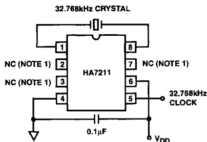
32.768kHz MICROPOWER CLOCK OSCILLATOR
