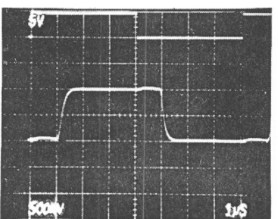
SMALL-SIGNAL SWITCHING WITH FILTERING
