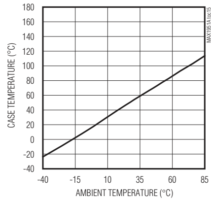
CASE TEMPERATURE vs. AMBIENT TEMPERATURE
