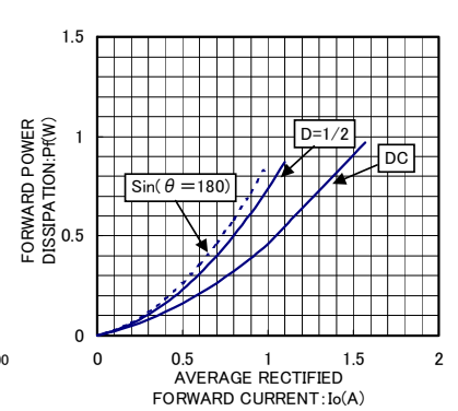
Io-Pf CHARACTERISTICS
