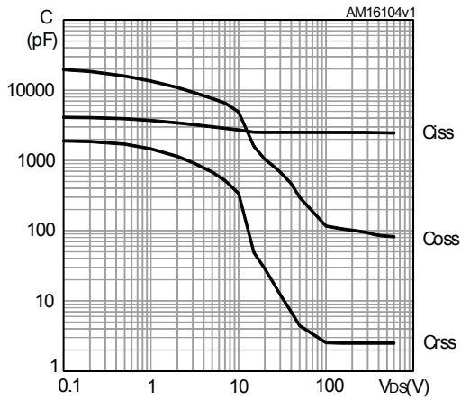
Figure 7. Capacitance variations
