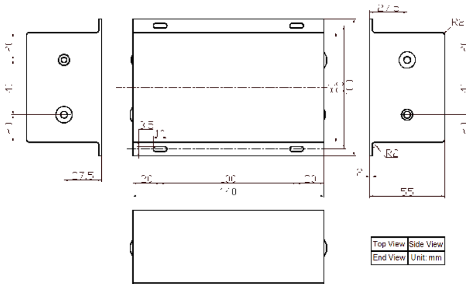
Figure 12. Dimensions for AHV24V25KV1MAW
