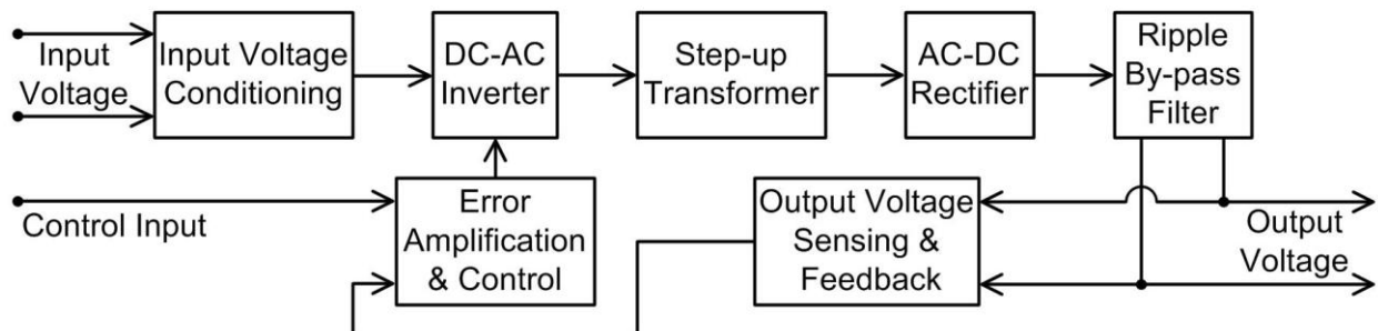
Figure 10. Block Diagram
