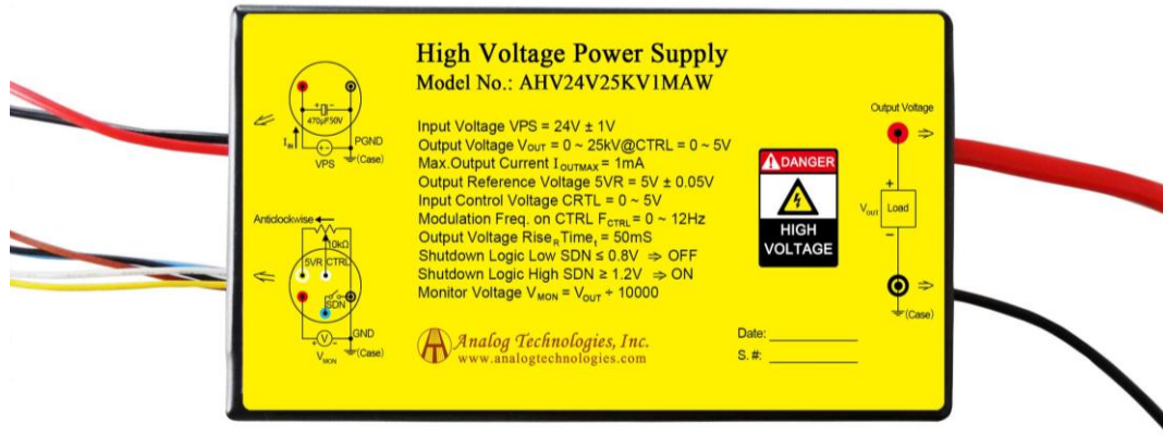
Figure 1. Physical Photo of AHV24V25KV1MAW
