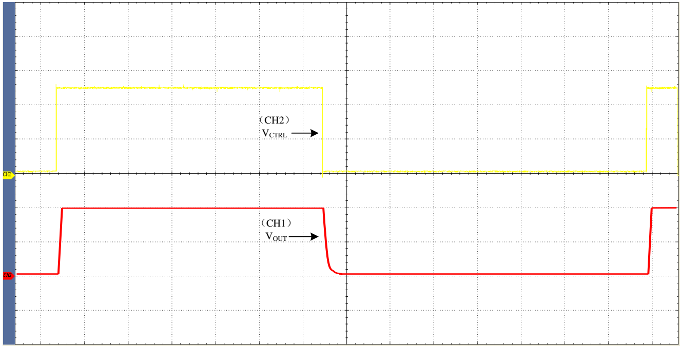
CH1: 12500V/Div CH2: 2V/Div M: 500ms V_{CTRL} : 0.25V ~ 5V V_{OUT} : 1250V ~ 25000V
