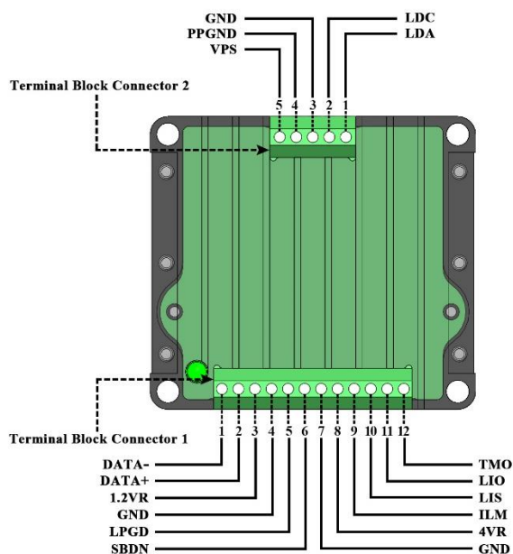
Figure 4. Top View of AQCL200MA410DF
