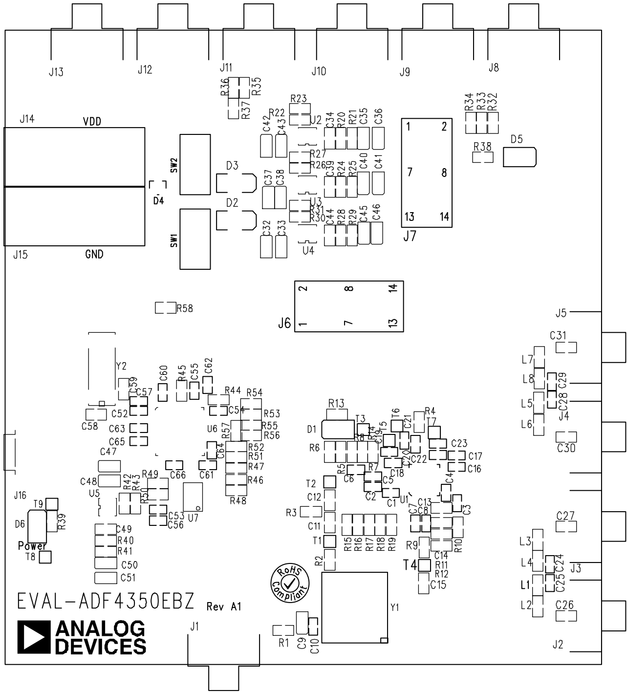
Figure 8. Evaluation Board Silk Screen
