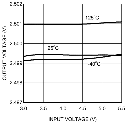
Figure 25. Line Regulation
