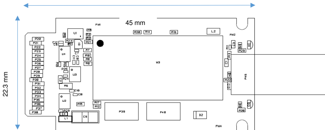
Figure 7: Mechanical drawing
