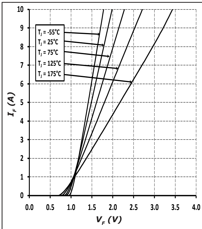
Figure 1. Forward Characteristics
