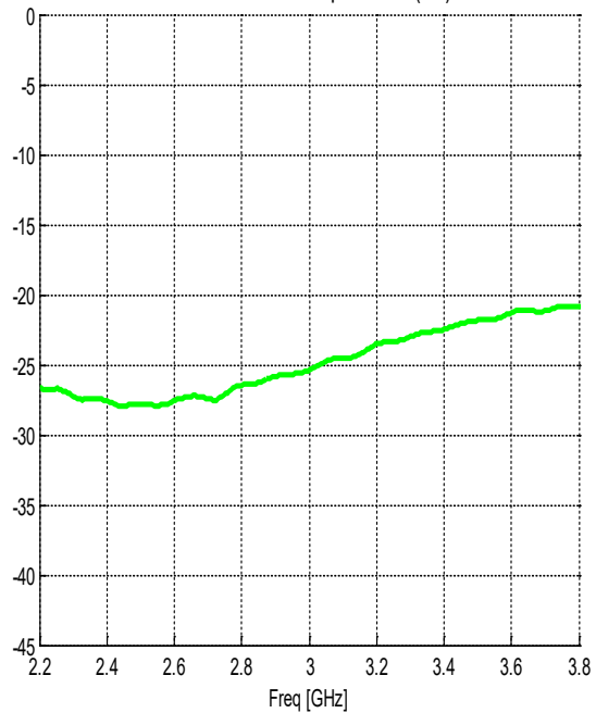
Return Loss at Coupled Port (dB)
