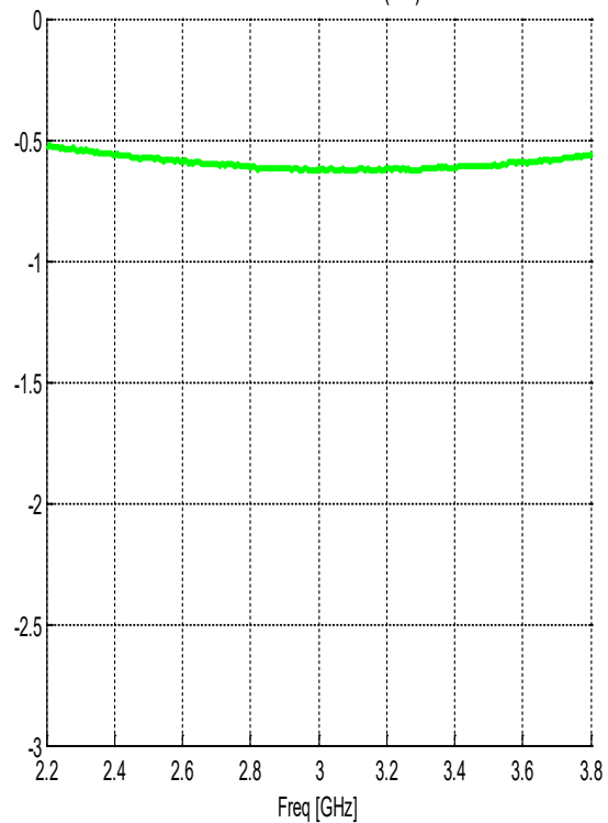
Transmission Loss (dB)
