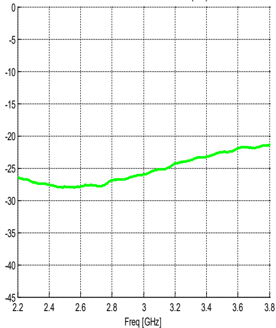
Return Loss at Isolated Port (dB)
