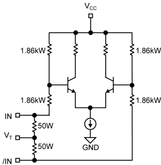
Figure 2a. Simplified Differential Input Buffer
