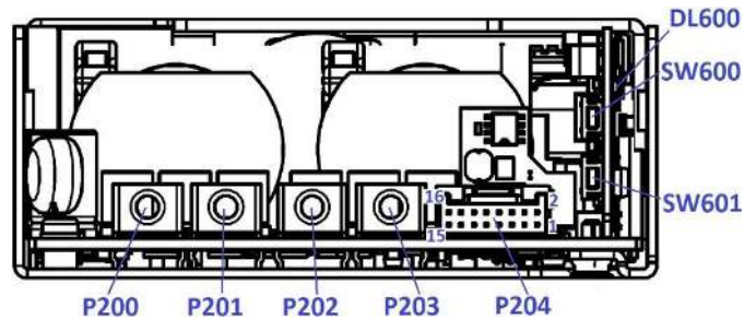
Figure 4. Rear View - ACC750-1T24 / ACC750-1T48 Models
