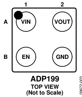
Figure 3. Pin Configuration
