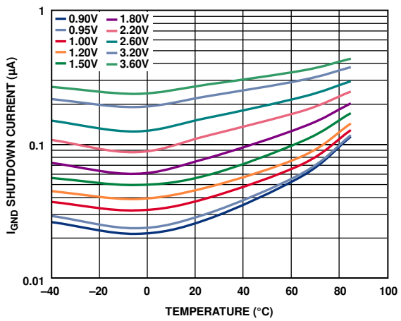
Figure 14. Ground Shutdown Current vs. Temperature, Output Open, Different Input Voltage ( V_{IN} )
