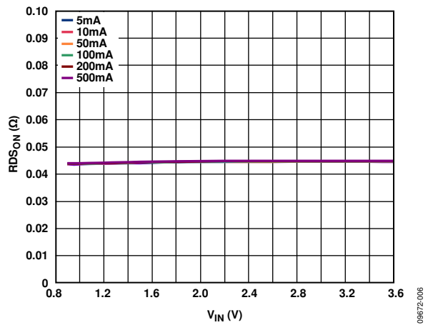
Figure 6. R_{DS\text{ON}} vs. Input Voltage ( V_{IN} ), Different Load Currents
