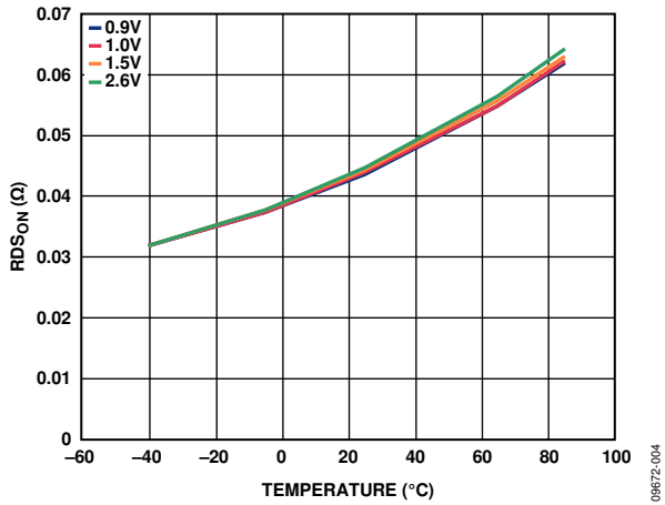
Figure 4. R_{DS\text{ON}} vs. Temperature, 50 mA, Different Input Voltage ( V_{IN} )
