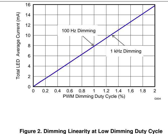
Figure 2. Dimming Linearity at Low Dimming Duty Cycle
