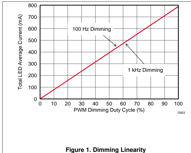
Figure 1. Dimming Linearity
