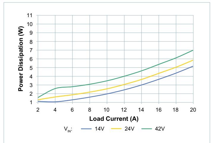
Figure 33 — System power dissipation, low trim, board temperature = 25°C
