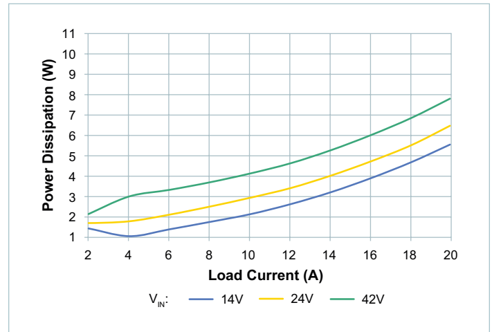
Figure 32 — System power dissipation, nominal trim, board temperature = 25°C
