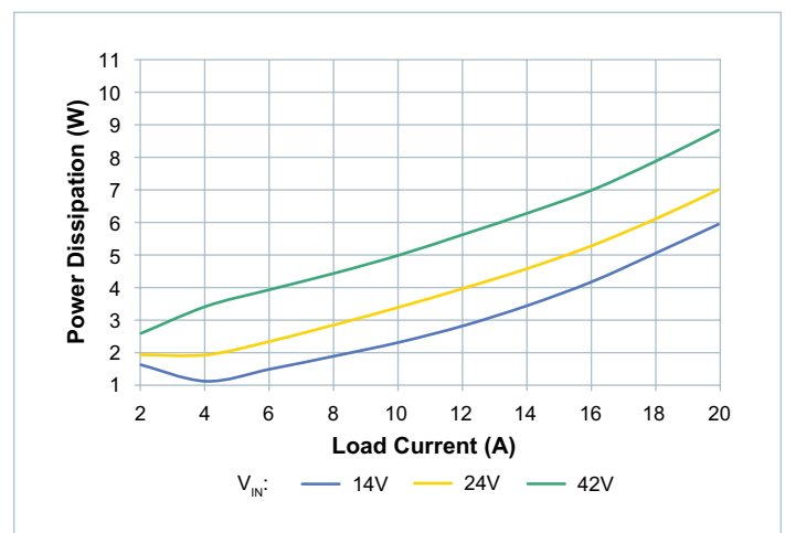
Figure 34 — System power dissipation, high trim, board temperature = 25°C
