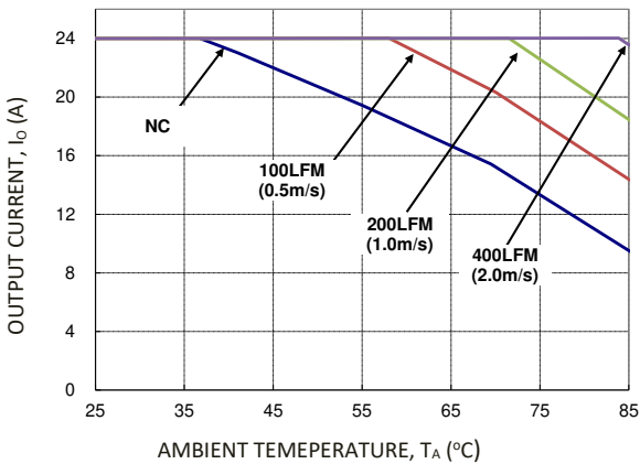
Figure 19. Output Current Derating for the Module with Heatplate; Airflow in the Transverse Direction from V out (-) to V out (+); V IN =24V, V O =5V.
