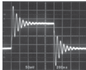
R_F = 1k V_S = \pm 15V f = 500kHz LT1222 • TPC24 R_G = 100\Omega (75) V_{IN} = 15mV
