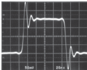
R_F = 909\Omega V_S = \pm 15V f = 5MHz LT1222 • TPC19 R_G = 100\Omega V_{IN} = 20mV
