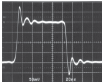
R_F = 1k V_S = \pm 15V f = 5MHz LT1222 • TPC22 R_G = 100\Omega (75) V_{IN} = 20mV
