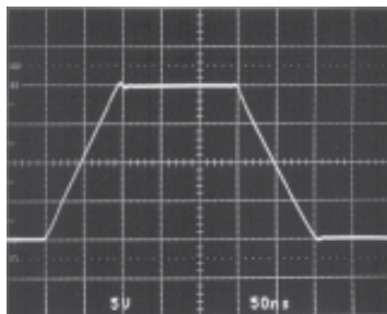
R_F = 1k V_S = \pm 15V f = 2MHz LT1222 • TPC23 R_G = 100\Omega (75) V_{IN} = 2V
