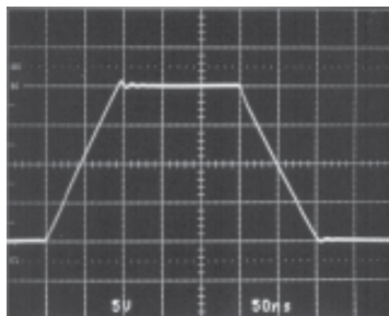
R_F = 909\Omega V_S = \pm 15V f = 2MHz LT1222 • TPC20 R_G = 100\Omega V_{IN} = 2V
