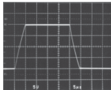
R_F = 909\Omega V_S = \pm 15V f = 20kHz LT1222 • TPC21 R_G = 100\Omega V_{IN} = 2V
