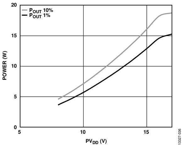
Figure 44. Output Power vs. P_{VDD} , R_L = 8 \Omega , Analog Gain = 15
