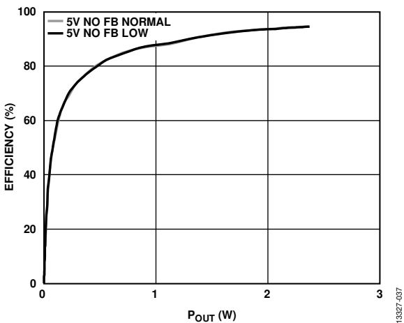
Figure 45. Efficiency vs. P_{OUT} , R_L = 8 \Omega , No FB and 220 pF Capacitor, P_{VDD} = 5 V , Analog Gain = 8.4
