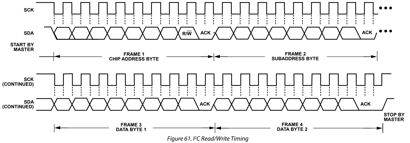
Figure 61. I 2 C Read/Write Timing
