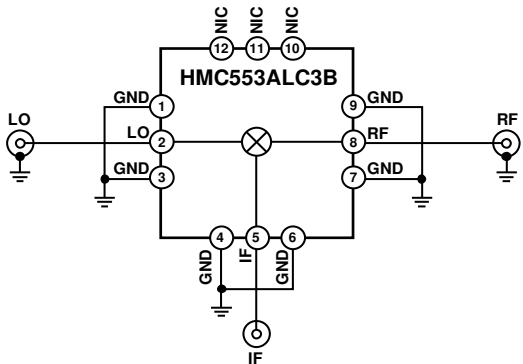
Figure 82. Typical Application Circuit
