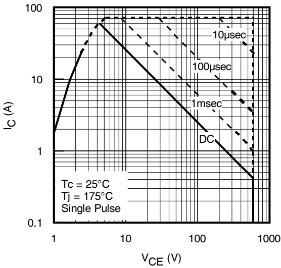
Fig. 3 - Forward SOA
