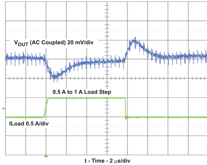
Figure 3-11. Load Transient Response With 2.2-μH Inductor and Vin = 12 V
