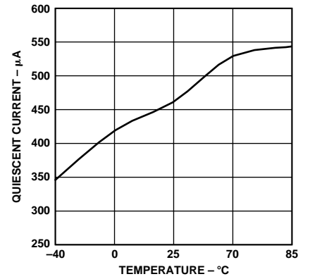
Figure 11. Quiescent Current vs. Temperature
