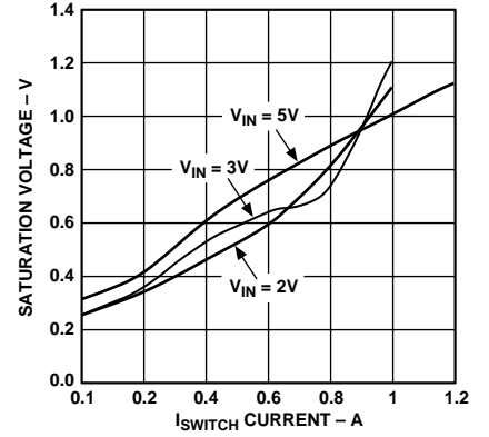
Figure 8. Saturation Voltage vs. I_{SWITCH} Current in Step-Up Mode
