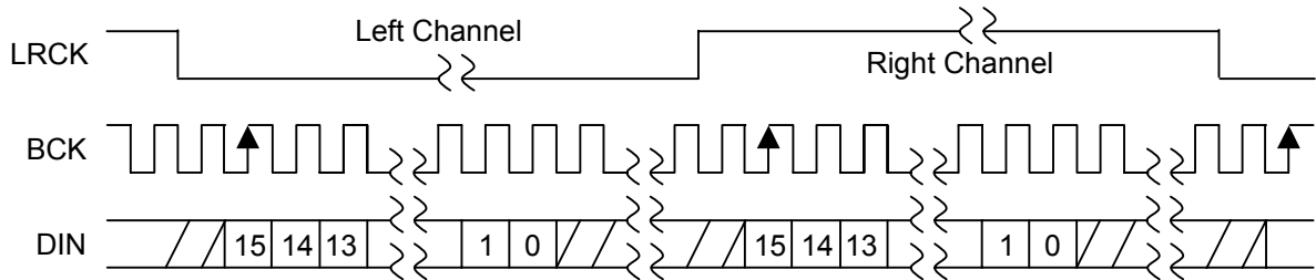
Figure 3.1. 16 bits I 2 S Data Format
