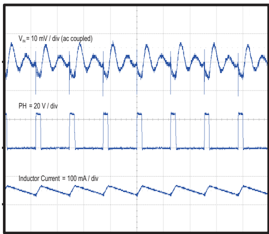
Figure 31. Input Ripple in CCM
