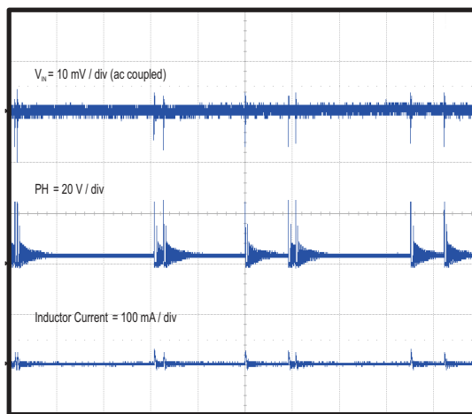
Figure 32. Input Ripple Skip
