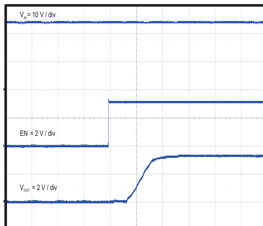
Figure 28. Start-Up With ENA
