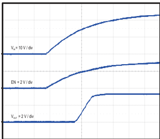
Figure 29. Start-Up With V_{IN}
