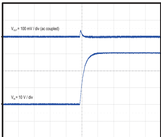
Figure 27. Line Transient
