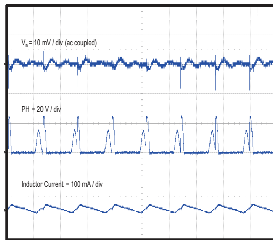
Figure 30. Input Ripple in DCM
