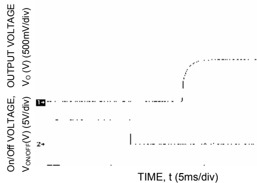
Figure 48. Typical Start-Up Using Remote On/Off, negative logic version shown.
