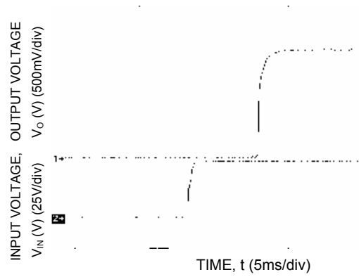
Figure 29. Typical Start-Up with application of Vin.
