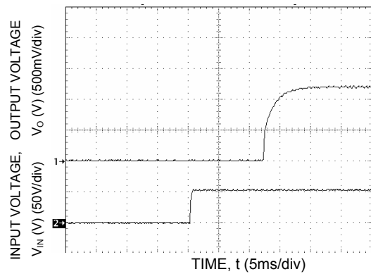
Figure 41. Typical Start-Up with application of Vin.
