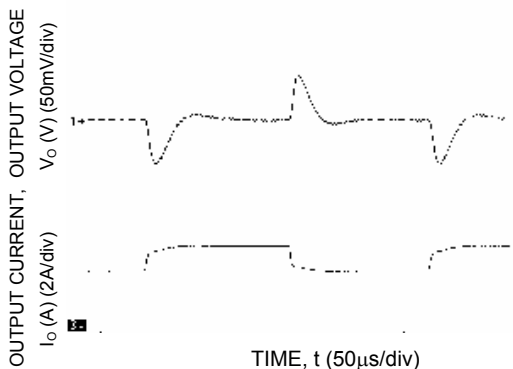
Figure 45. Transient Response to Dynamic Load Change from 50% to 75% to 50% of full load.
