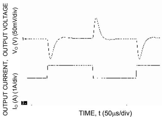
Figure 51. Transient Response to Dynamic Load Change from 50% to 75% to 50% of full load.
