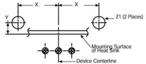
Mounting Details:
