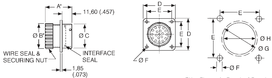
Panel Cutout
