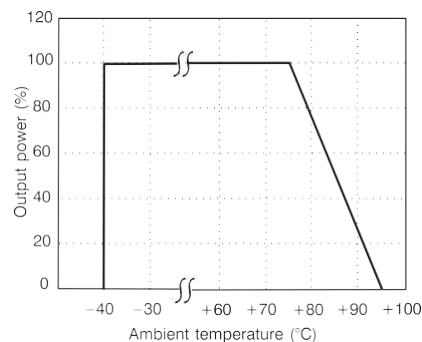
Power derating
