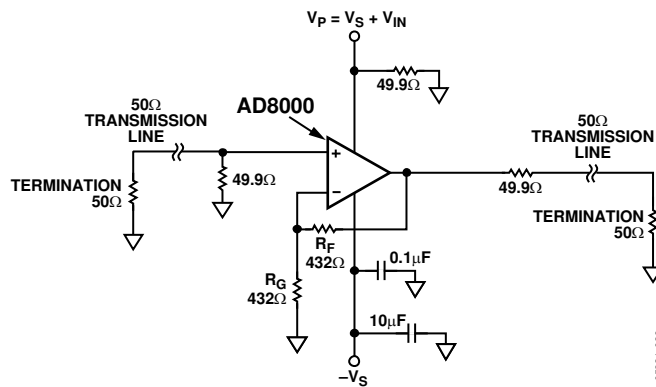
Figure 48. Positive PSRR
