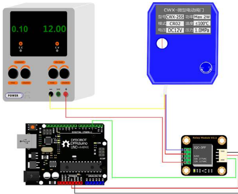
FIT0616-Arduino Connection Diagram
