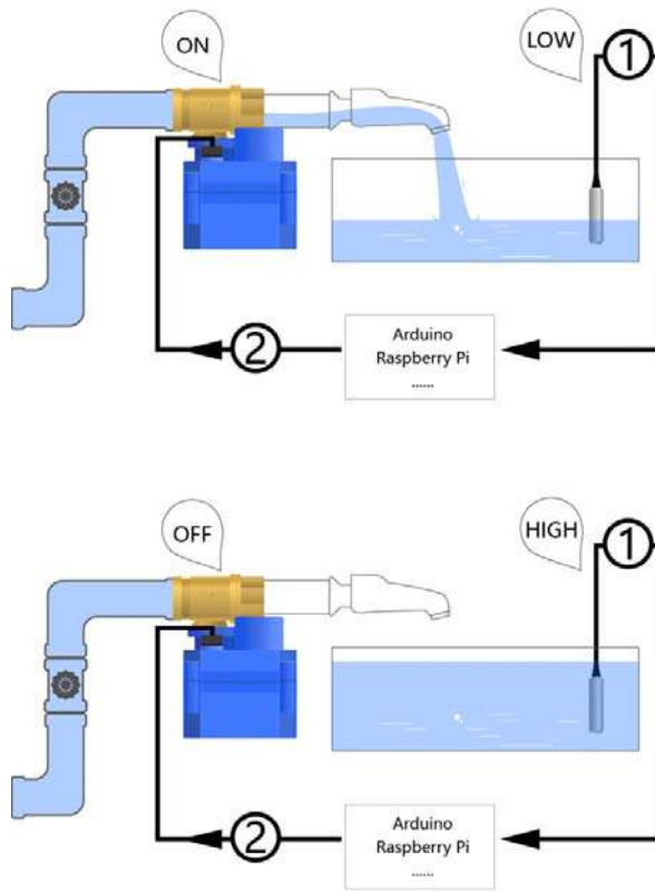
Smart Water Tank Diagram (FIT0616+KIT0139)
