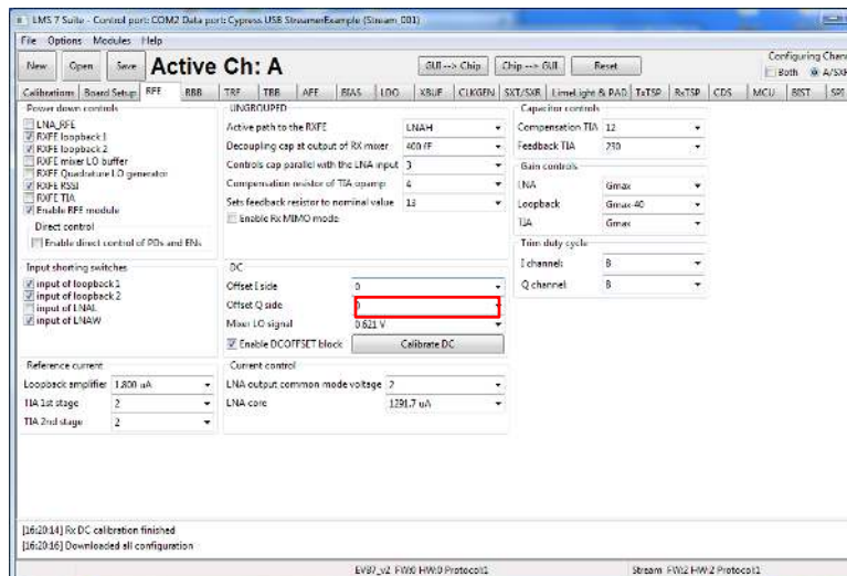
Figure 27 Calibrate RX DC offset
