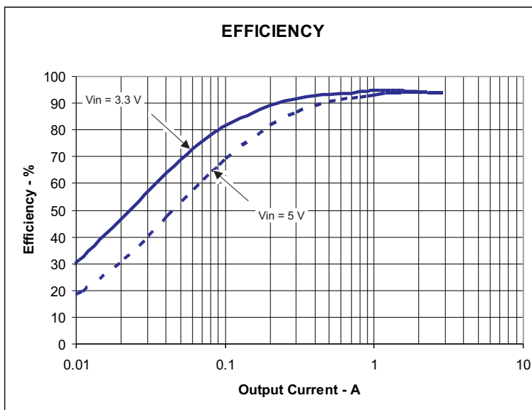
Figure 2. TPS54618EVM-606 Low Current Efficiency
