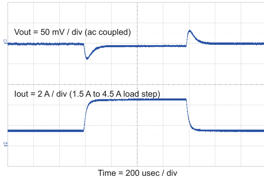
Figure 5. TPS54618EVM-606 Transient Response
