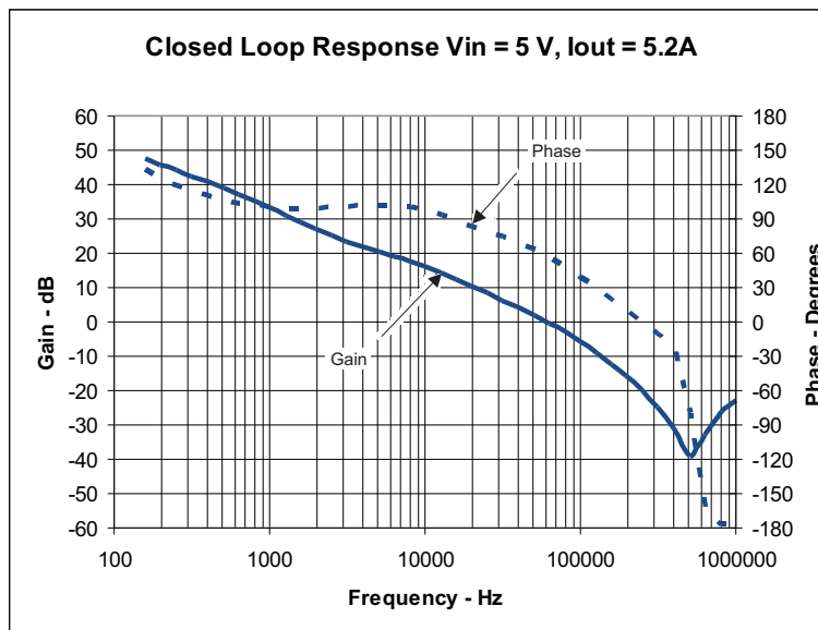
Figure 6. TPS54618EVM-606 Loop Response
