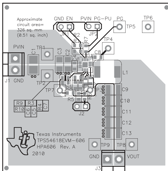
Figure 15. TPS54618EVM-606 Top-Side Assembly
