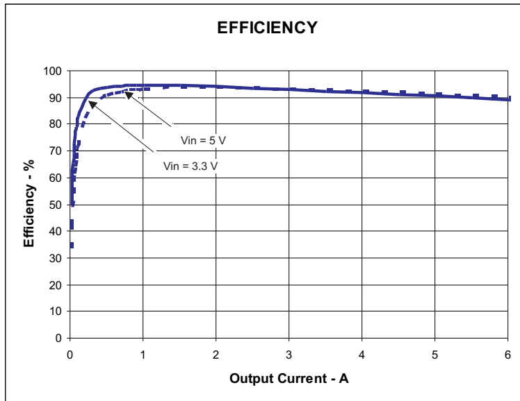
Figure 1. TPS54618EVM-606 Efficiency
