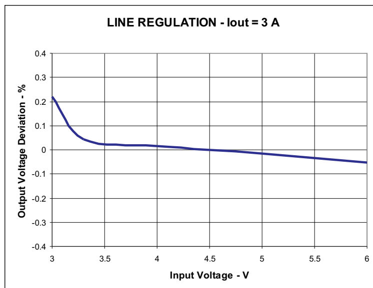
Figure 4. TPS54618EVM-606 Line Regulation
