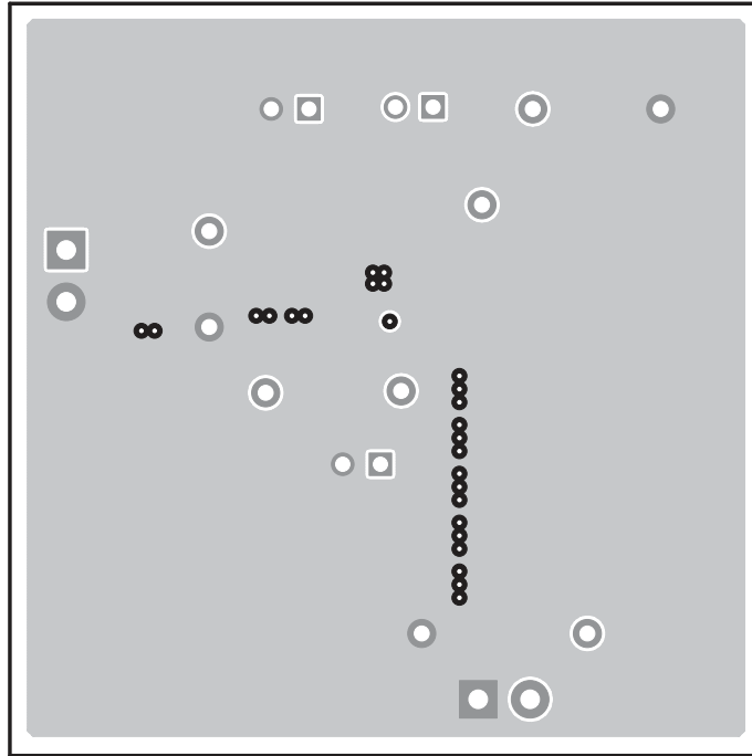
Figure 12. TPS54618EVM-606 Bottom-Side Layout
