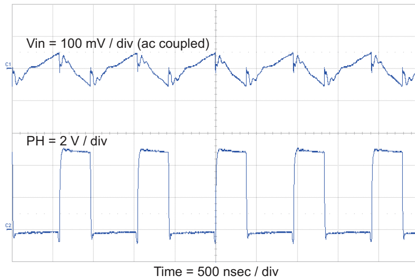
Figure 8. TPS54618EVM-606 Input Ripple
