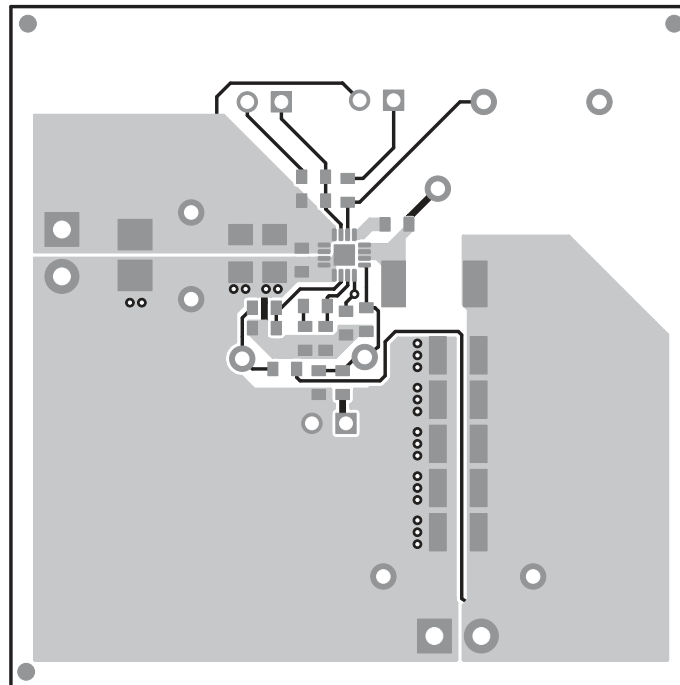
Figure 11. TPS54618EVM-606 Top-Side Layout
