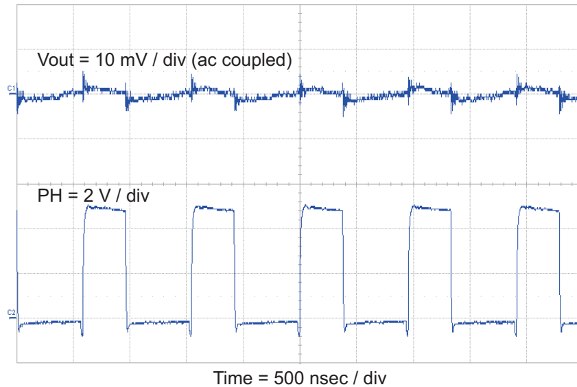
Figure 7. TPS54618EVM-606 Output Ripple
