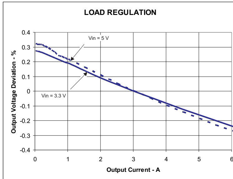
Figure 3. TPS54618EVM-606 Load Regulation
