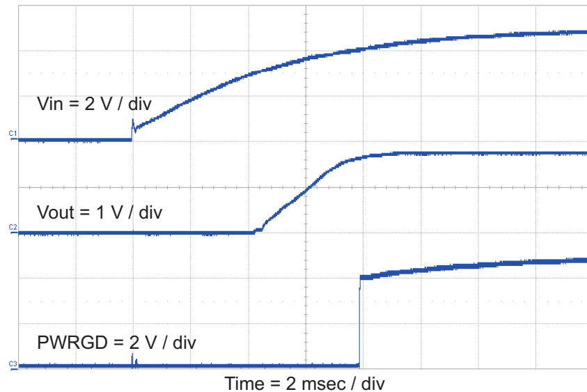
Figure 9. TPS54618EVM-606 Start-Up Relative to V_{IN}
