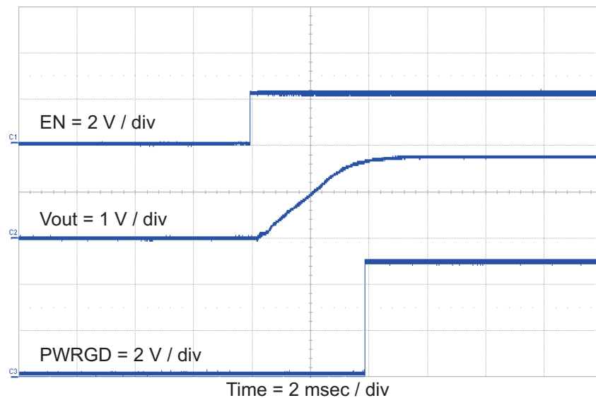
Figure 10. TPS54618EVM-606 Start-Up Relative to Enable
