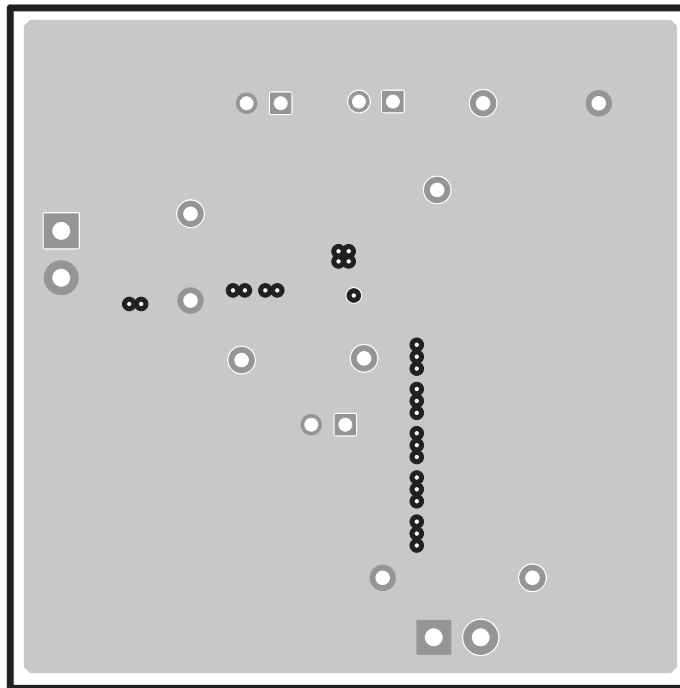
Figure 13. TPS54618EVM-606 Internal Layer 1
