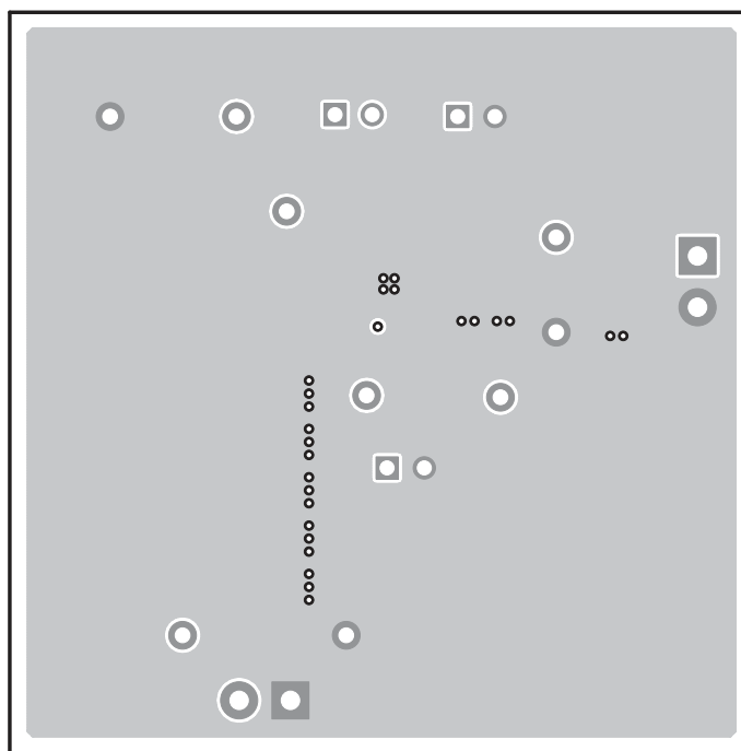
Figure 14. TPS54618EVM-606 Internal Layer 2
