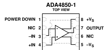
Figure 1. 8-Lead, 3 mm × 3 mm LFCSP
