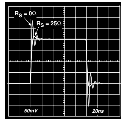
Figure 6. Capacitive Load Drive
