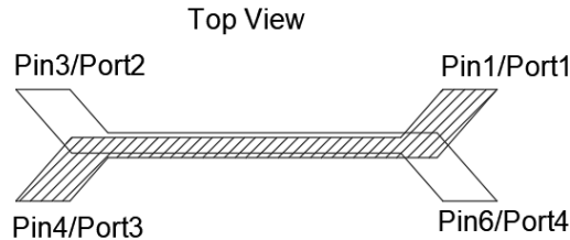
0603 size 5dB Coupler Pin Configuration
